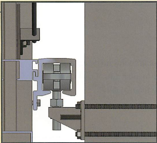
BOTTOM SUPPORT RAIL (CUT-AWAY VIEW)
