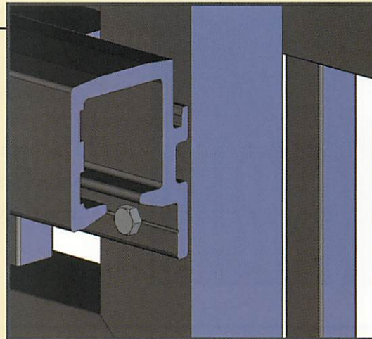
BOTTOM SUPPORT RAIL
